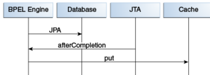
Figure 17-1 Dehydration Process
