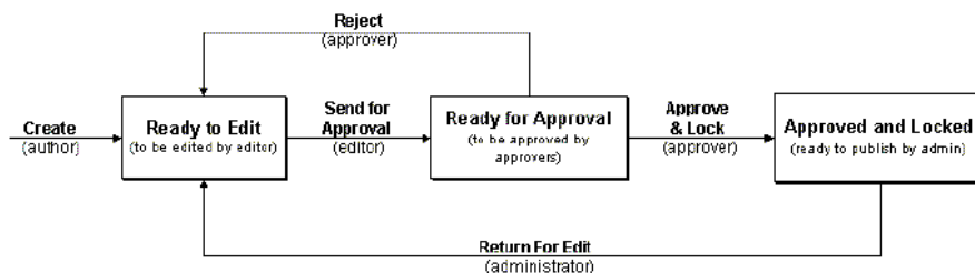
Figure 9-2 Workflow-Flowchart
