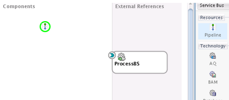
Figure 4-24 Pipeline Template
