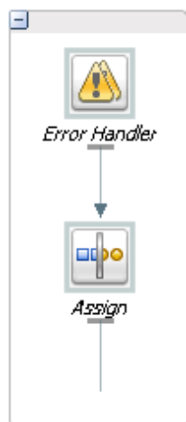
Figure 10-10 Error Handler
