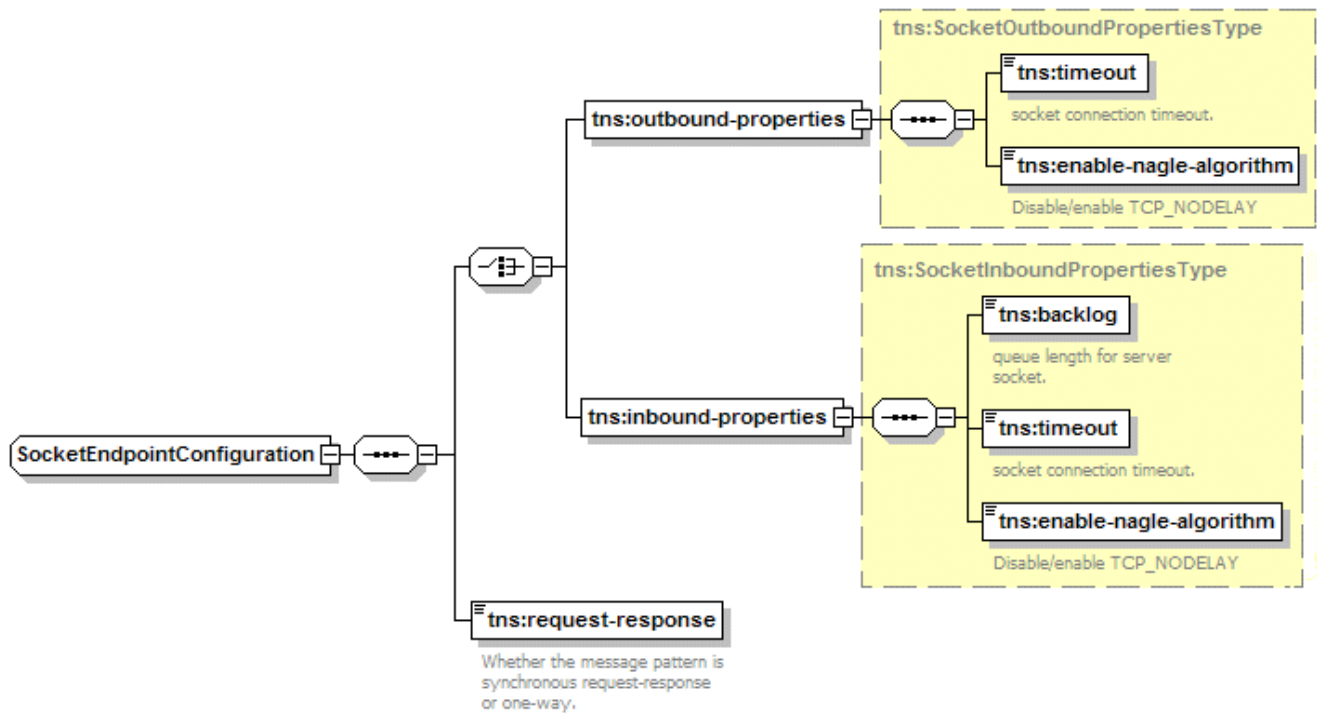
Figure 43-2 SocketEndpointConfiguration Properties
