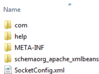
Figure 42-1 Plug-In Packaging
