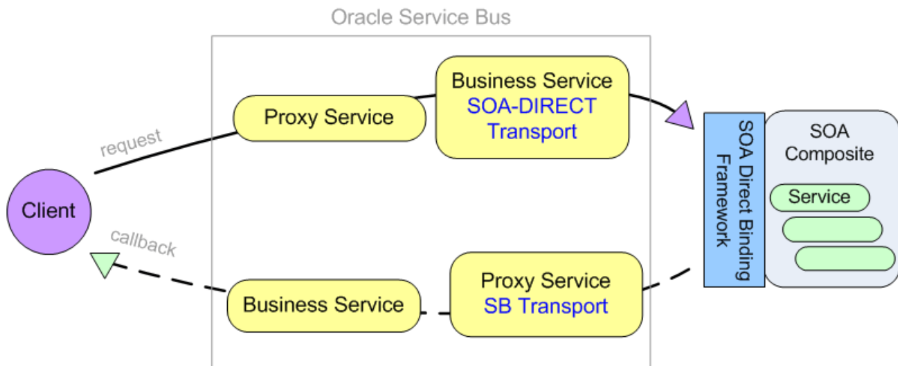
Figure 36-3 Client Invoking a SOA Binding Service Asynchronously
