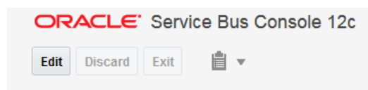
Figure 2-6 Sessions Toolbar
