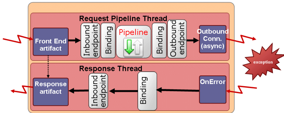
Figure 40-3 Error Case 2
