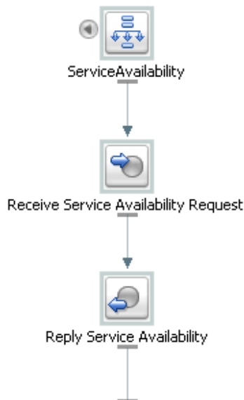
Figure 10-5 New Split-Join
