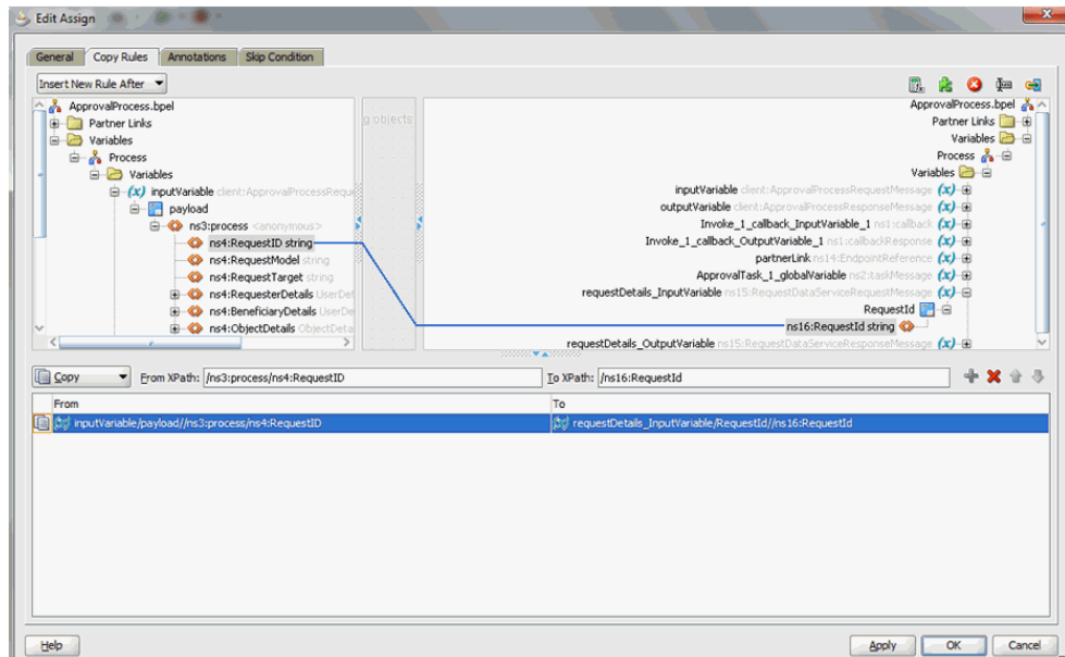
Figure 11-7 Input Mapping
