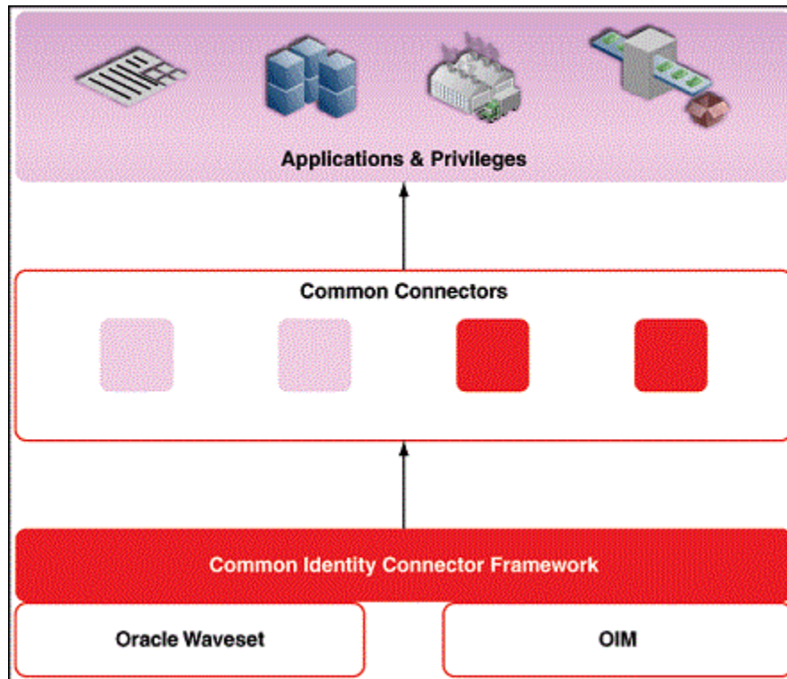
Figure 4-5 ICF Framework
