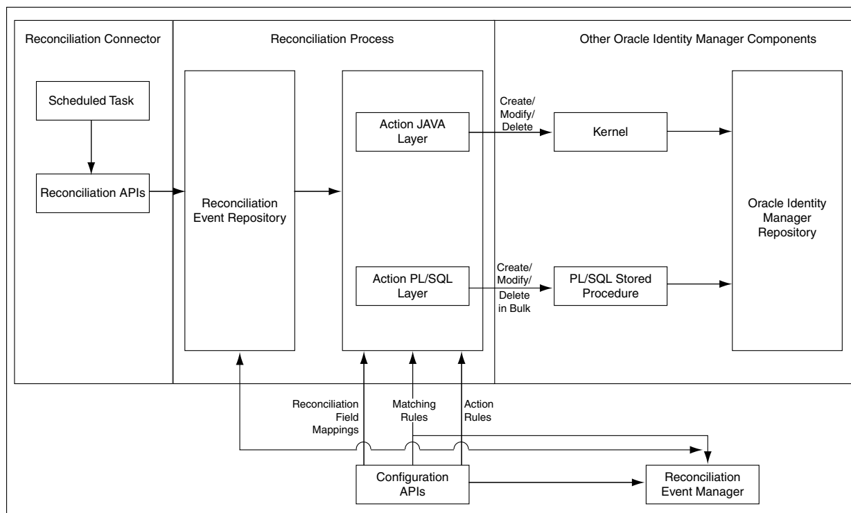
Figure 12-1 Reconciliation Architecture
