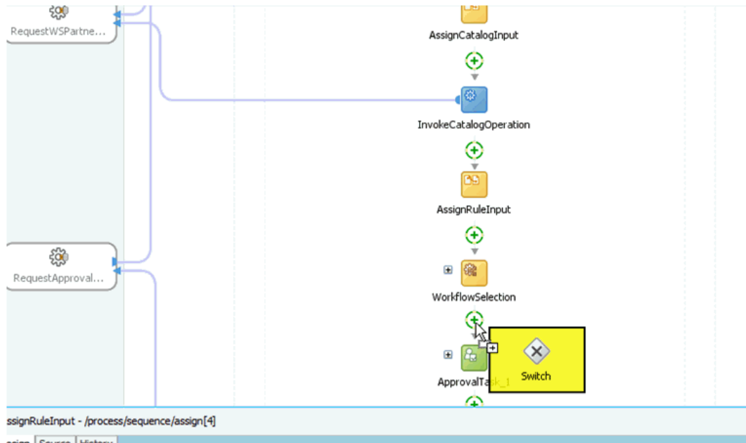
Figure 11-19 Switch Activity
