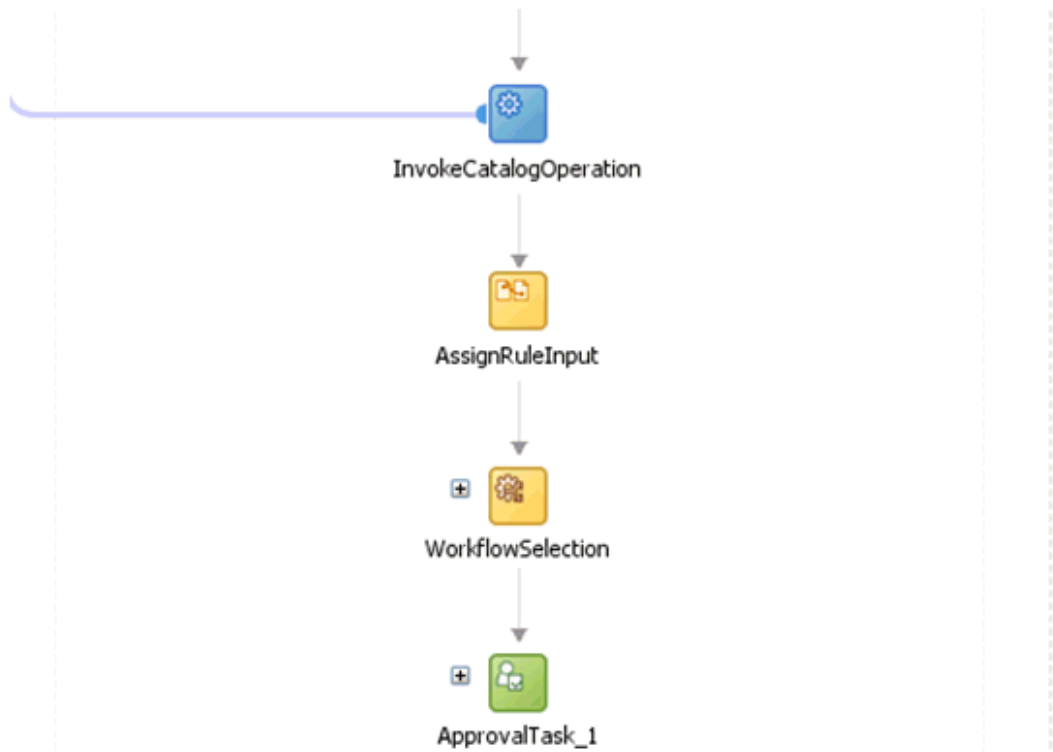
Figure 11-15 AssignRuleInput
