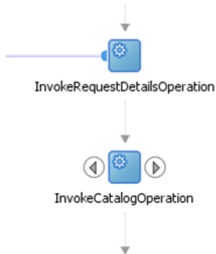
Figure 11-8 InvokeCatalogOperation
