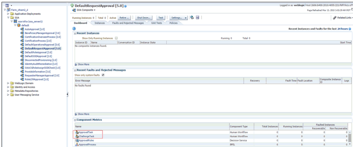
Figure 17-14 Human Tasks
