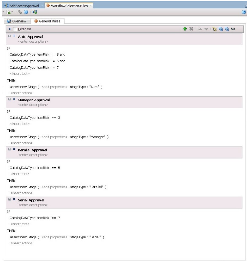
Figure 11-18 Approval Rules
