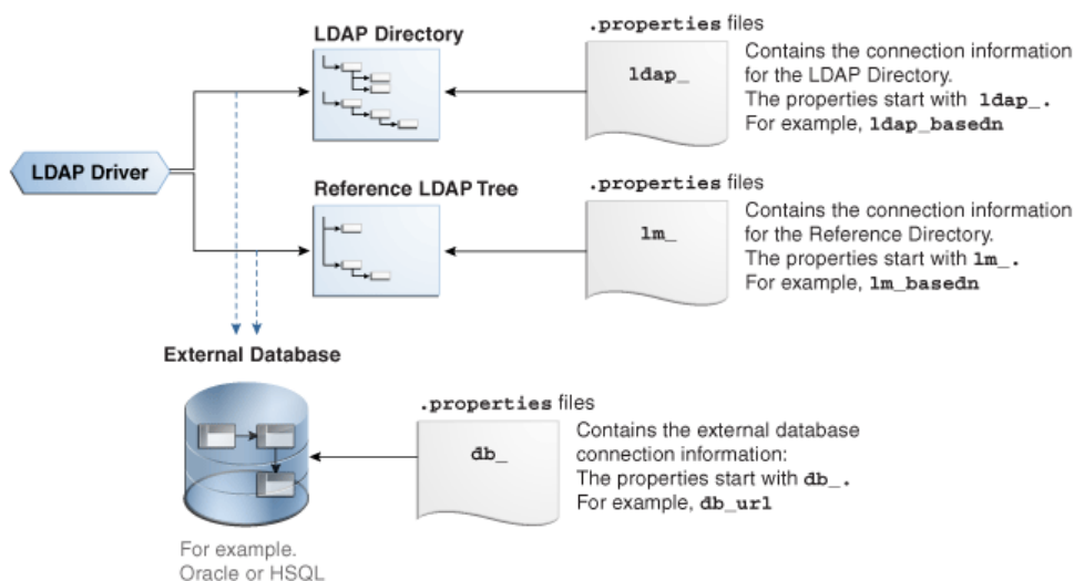
Figure A-3 Properties Files for LDAP Driver
