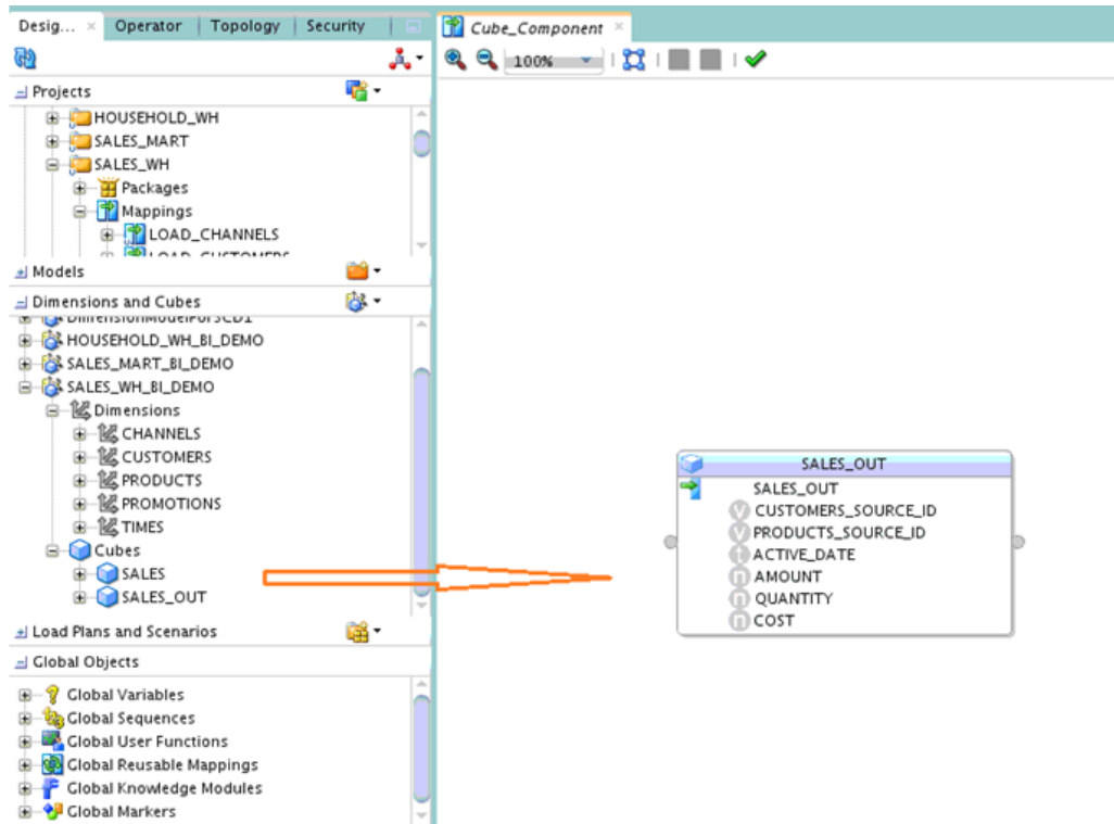
Figure 9-7 Using Cube Component in Mappings
