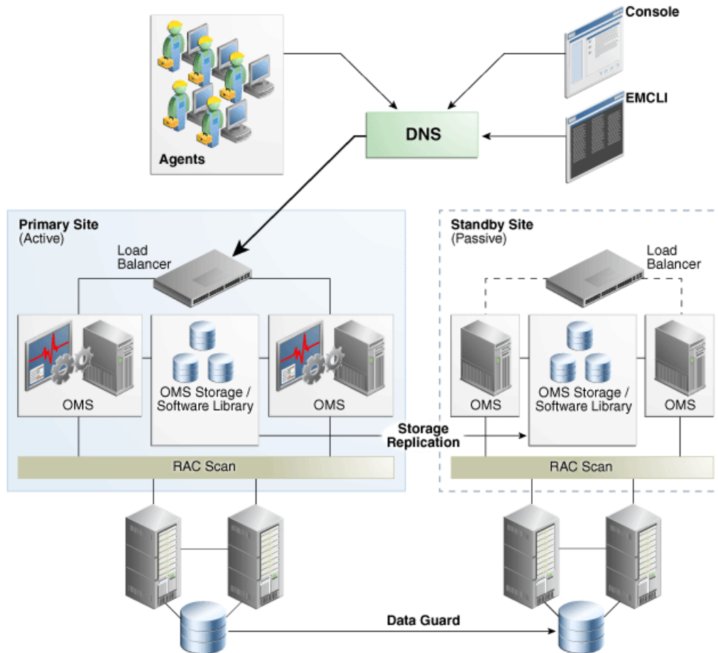
Figure 24-1 High Availability with Disaster Recovery Topology
