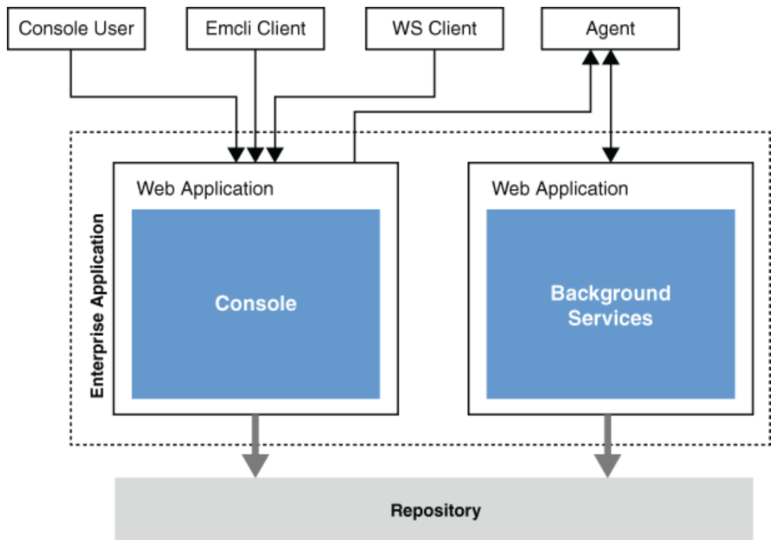
Figure 19-1 Functioning of OMS with Active Console and Background Services
