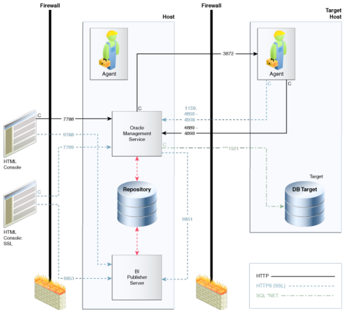
Figure 12-1 Firewall Port Requirements (Default)
