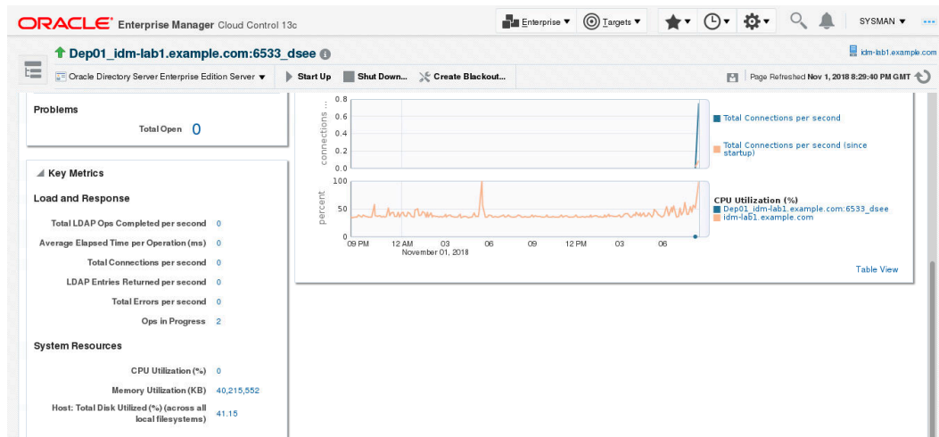
Figure 21-4 CPU Utilization Graph
