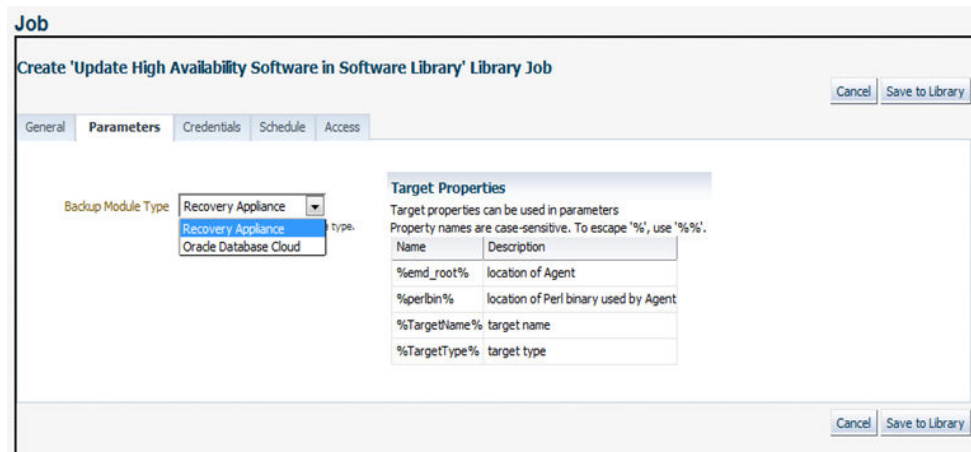
Figure 3-7 Create Library Job, Parameter Tab
