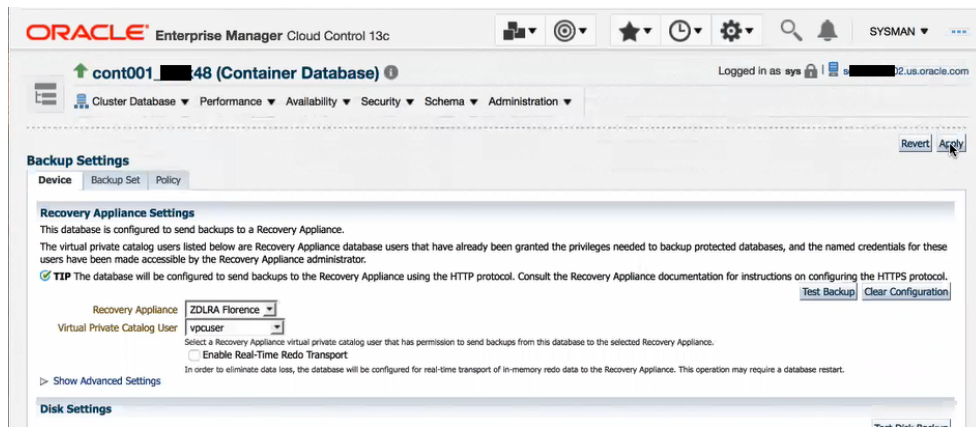
Figure 5-5 Enterprise Manager and turning off recovery protection
