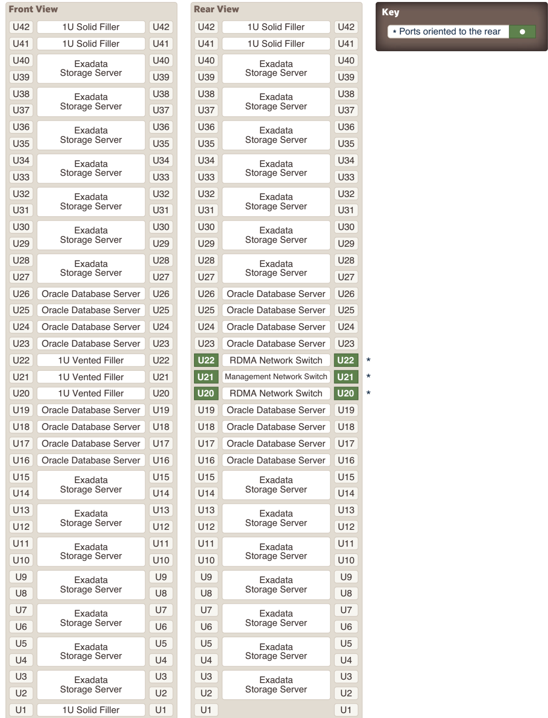
Figure 15-1 Rack Layout of Oracle Exadata X8M-2 Full Rack
