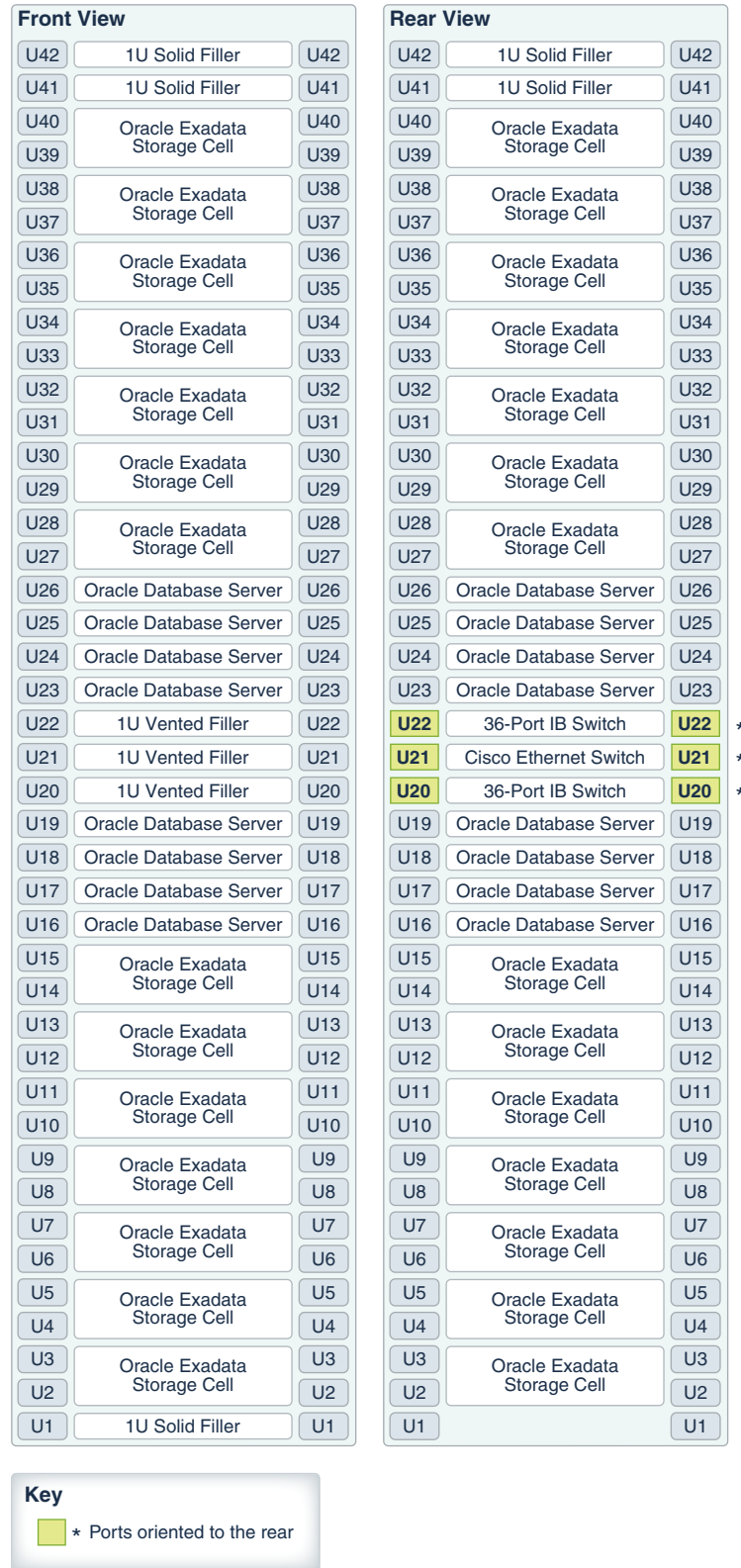
Figure 16-1 Rack Layout of Oracle Exadata Database Machine X8-2 and X7-2 Full Rack
