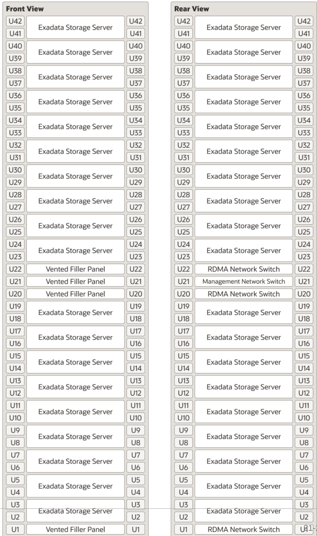
Figure 21-1 Rack Layout for Oracle Exadata Storage Expansion Rack X10M
