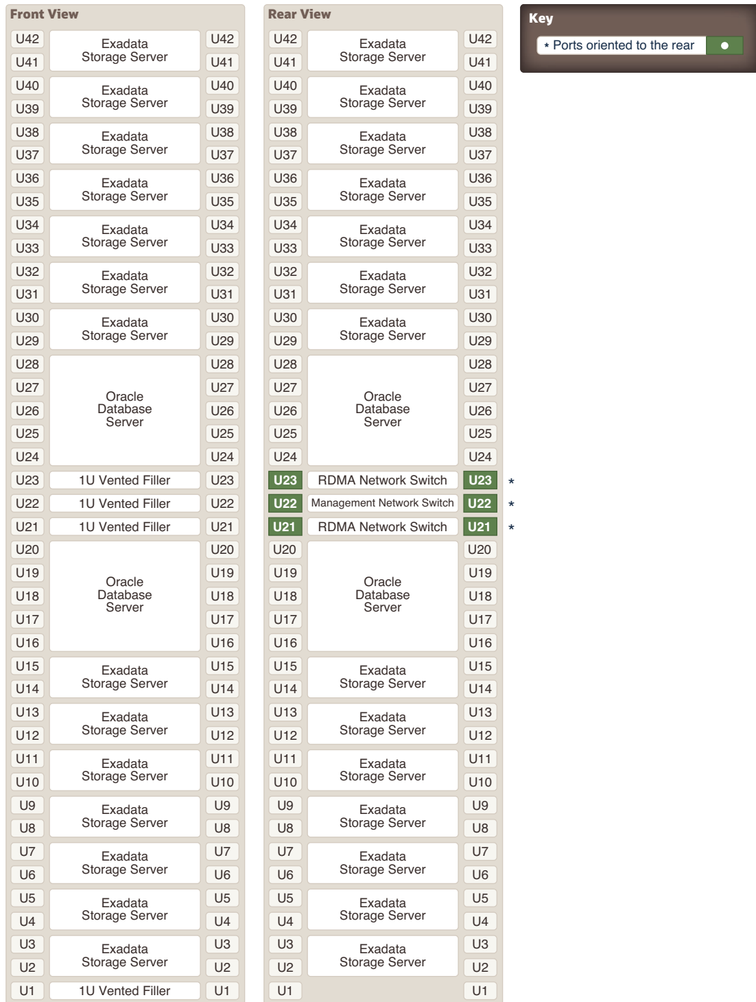
Figure 14-2 Rack Layout of Oracle Exadata X9M-8
