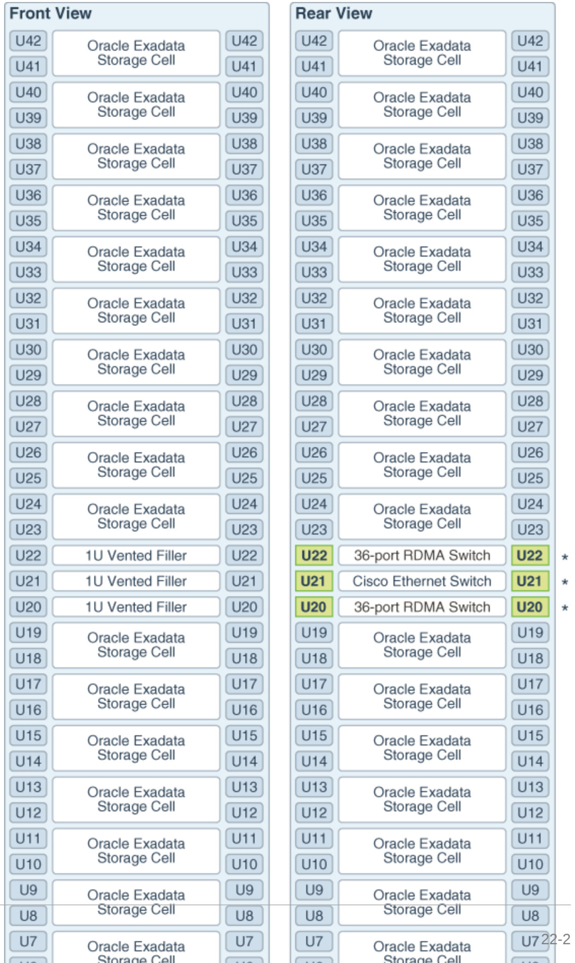
Figure 22-1 Rack Layout of Oracle Exadata Storage Expansion Rack X9M-2
