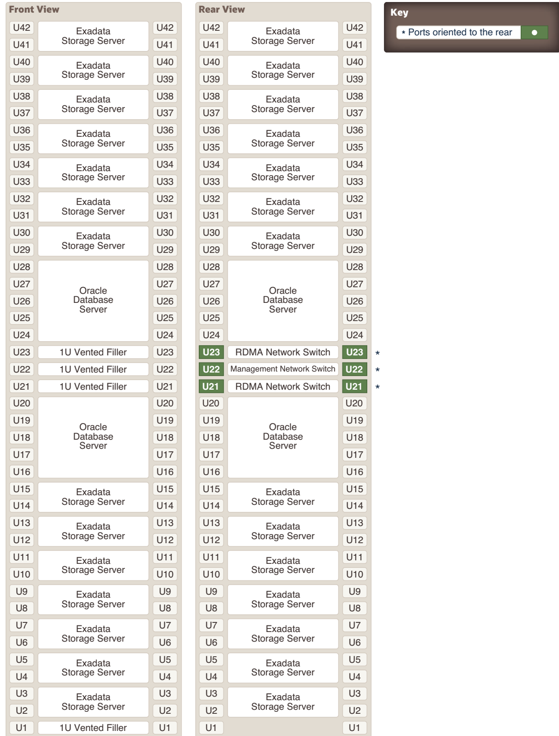
Figure 15-2 Rack Layout of Oracle Exadata X8M-8
