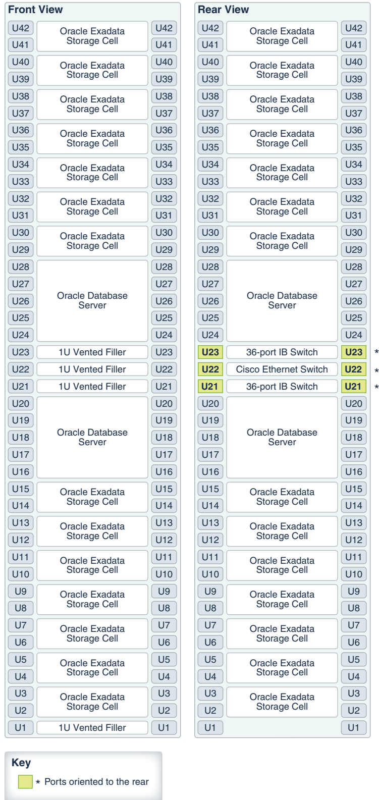
Figure 16-2 Rack Layout of Oracle Exadata Database Machine X8-8 and X7-8
