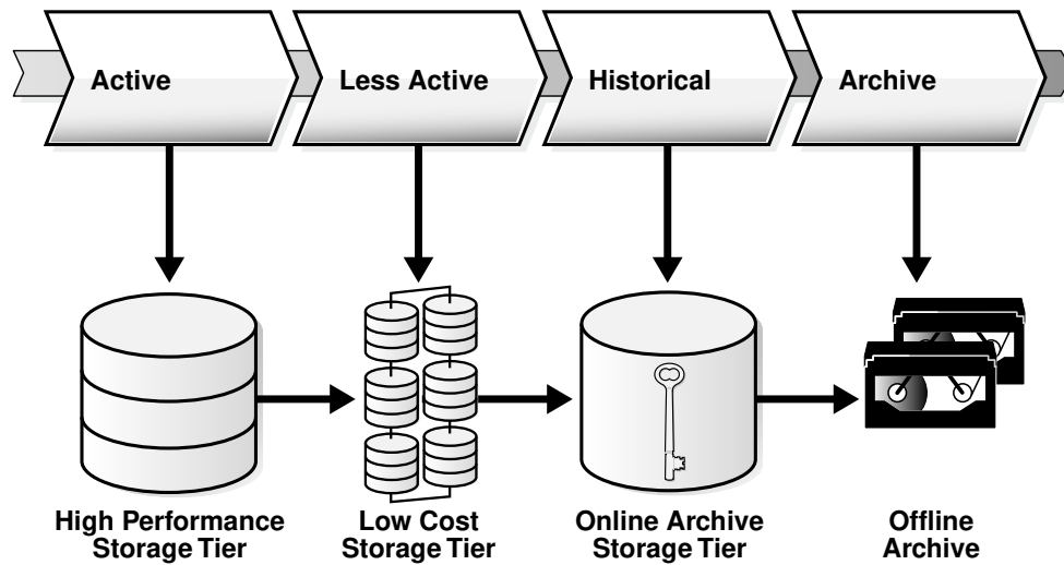
Figure 5-3 Data Lifecycle
