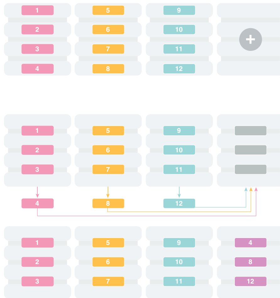
Figure 10-7 Resharding a Sharded Database
