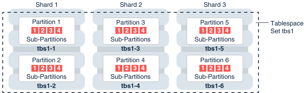
Figure 2-11 Subpartitions Stored in the Tablespace of the Parent Partition
