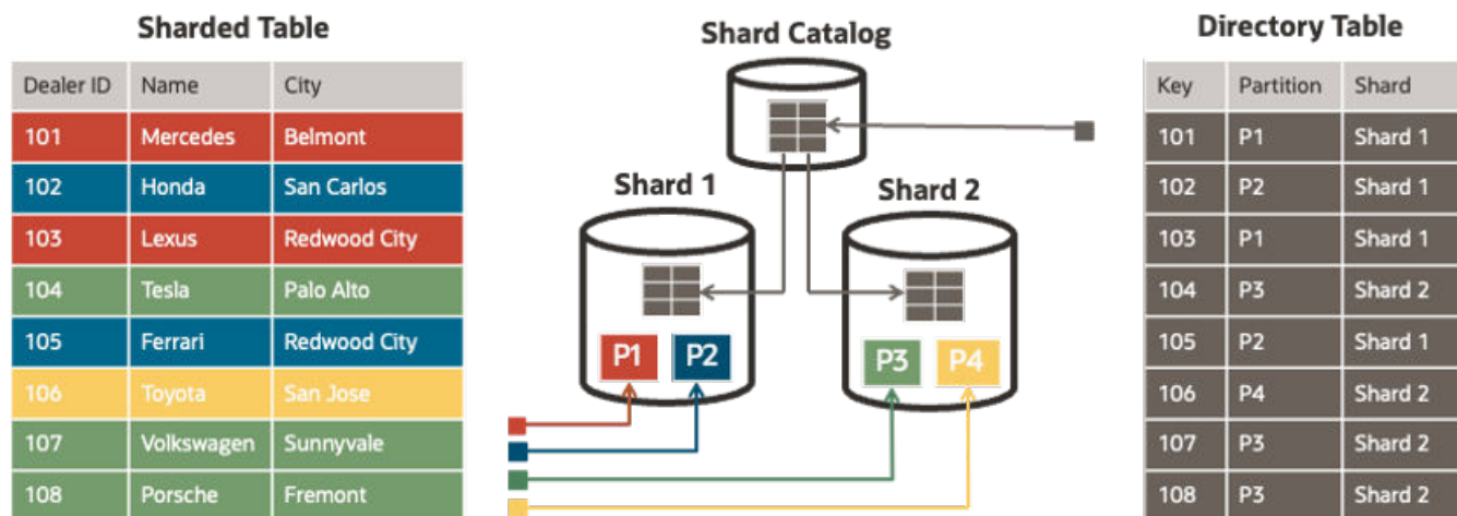
Figure 2-9 Directory-based sharding architecture
