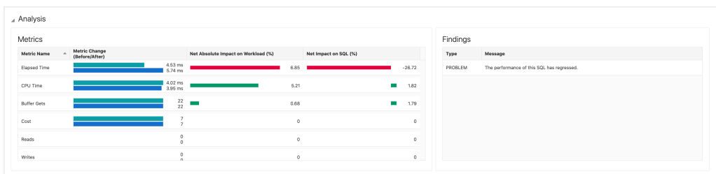
Figure 17-7 Analysis Metrics
