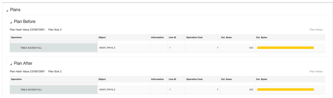
Figure 17-9 Plan Changes
