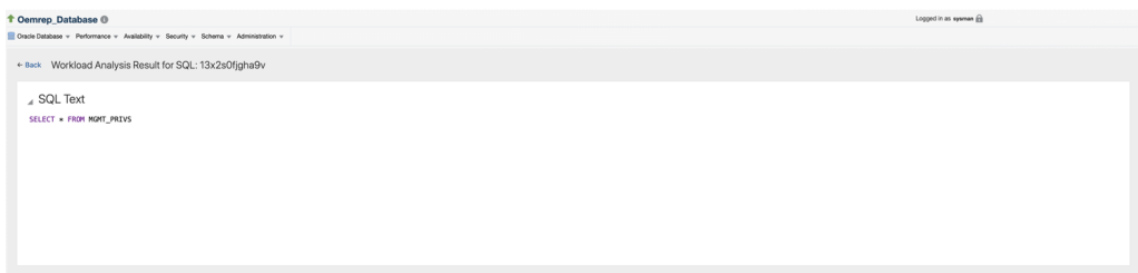
Figure 17-6 SQL Text
