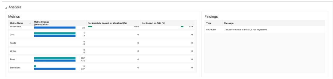
Figure 17-8 Analysis Findings
