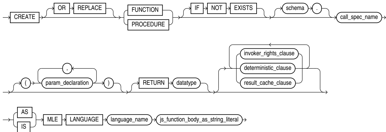
Figure 5-5 MLE Inlined Call Specification Syntax
