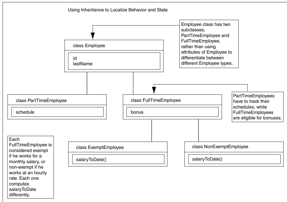
Figure 1-4 Class Hierarchy
