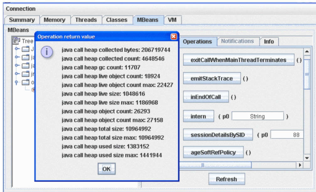
Figure 2-18 Operation sessionDetailsBySID
