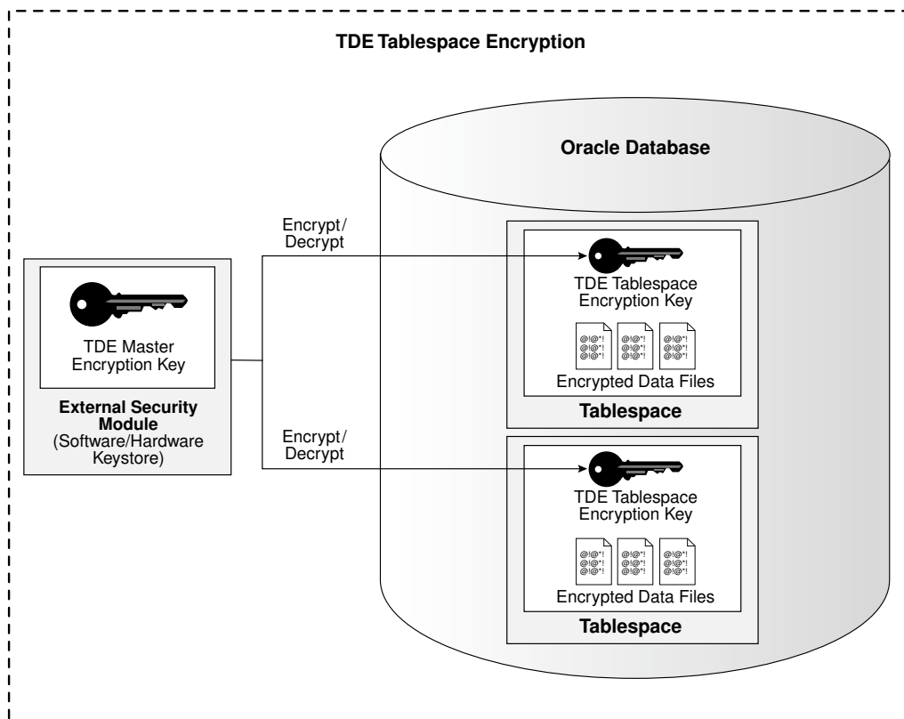
Figure 2-1 TDE Tablespace Encryption
