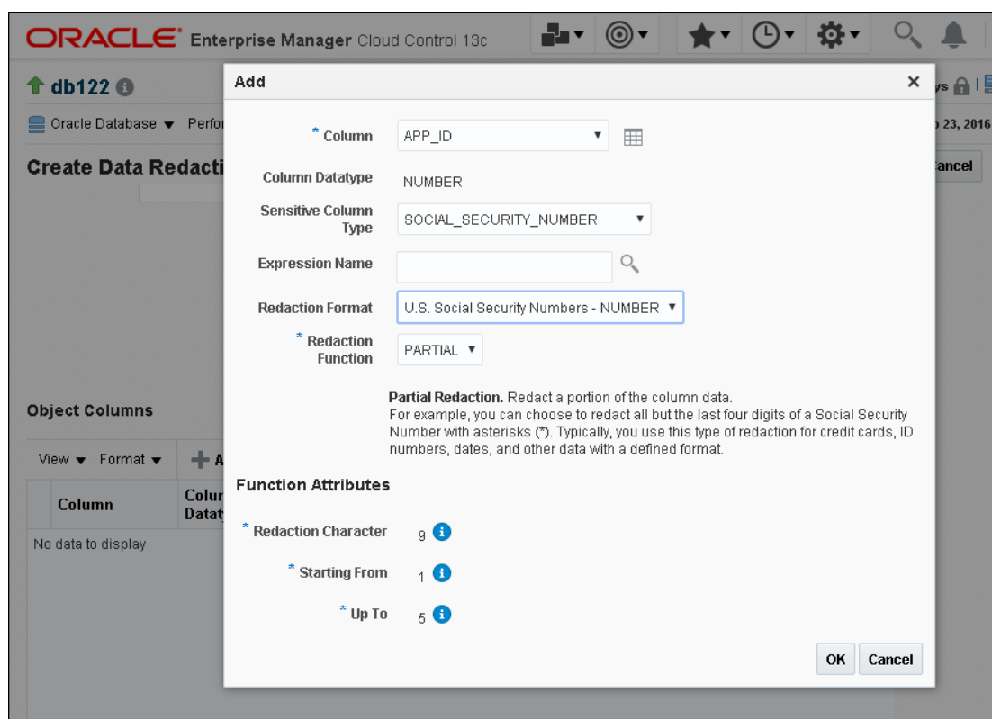
Figure 16-1 Oracle Data Redaction Formats Filtered on the Basis of Sensitive Column Types
