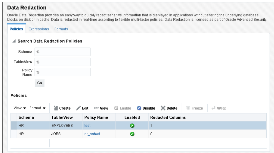
Figure 16-4 Oracle Data Redaction Policies Page
