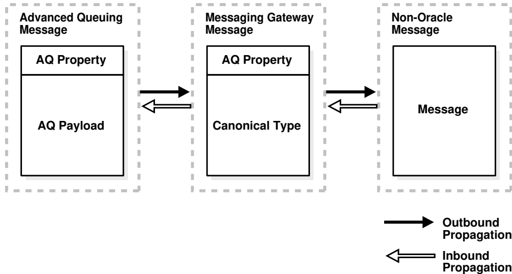
Figure C-2 Non-JMS Message Conversion
