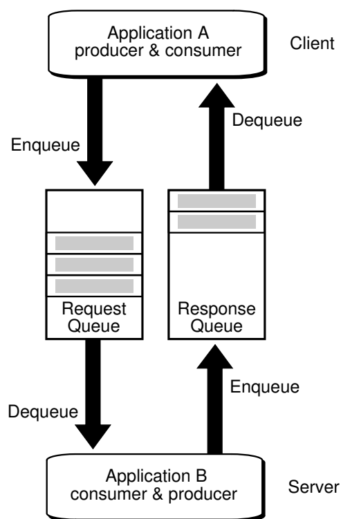
Figure 1-2 Client/Server Communication Using TxEventQ and AQ
