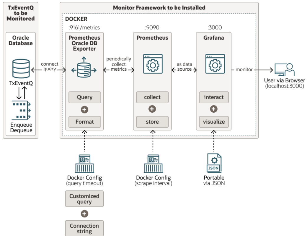
Figure 8-2 Monitoring Transaction Event Queue
