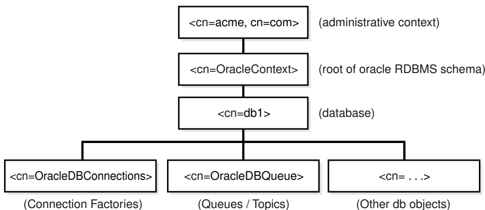
Figure 6-1 Structure of Oracle Database Advanced Queuing Entries in LDAP Server
