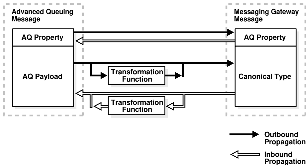
Figure C-3 Oracle Database Advanced Queuing Message Conversion
