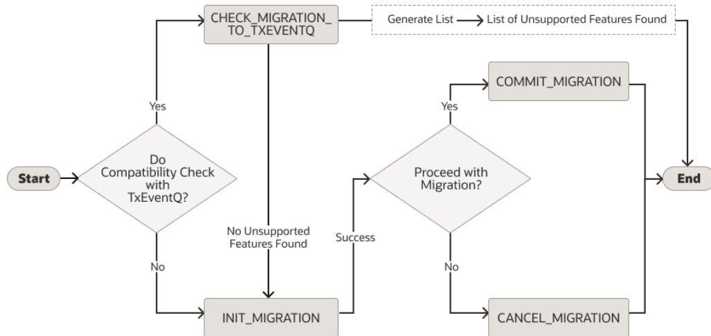
Figure 8-1 Flowchart: Migration from AQ to TxEventQ
