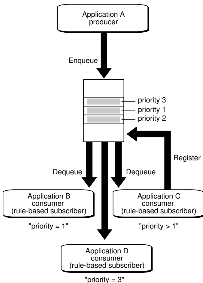
Figure 1-8 Implementing Publish/Subscribe using TxEventQ and AQ
