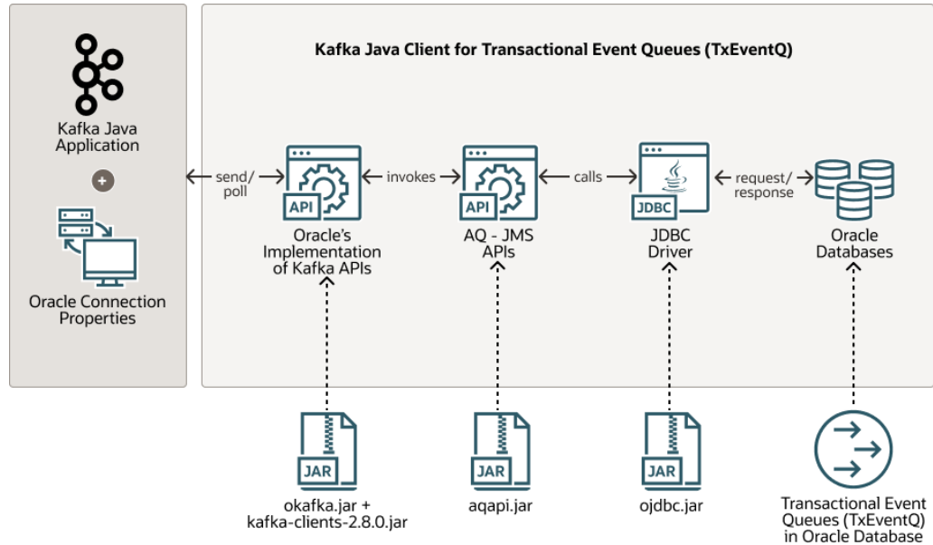
Figure 5-1 Kafka Application Integration with Transactional Event Queue
