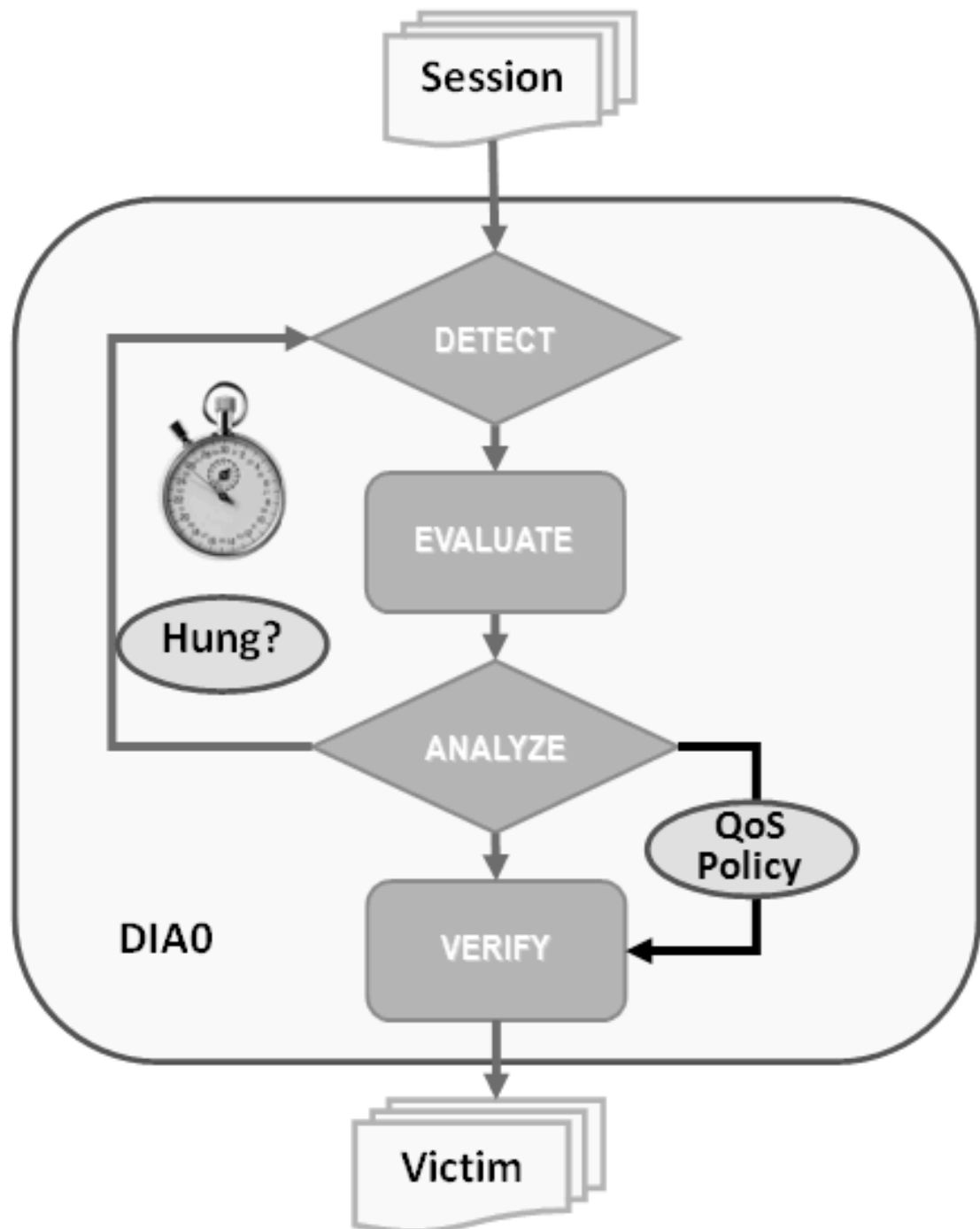
Figure 13-1 Hang Manager Architecture
