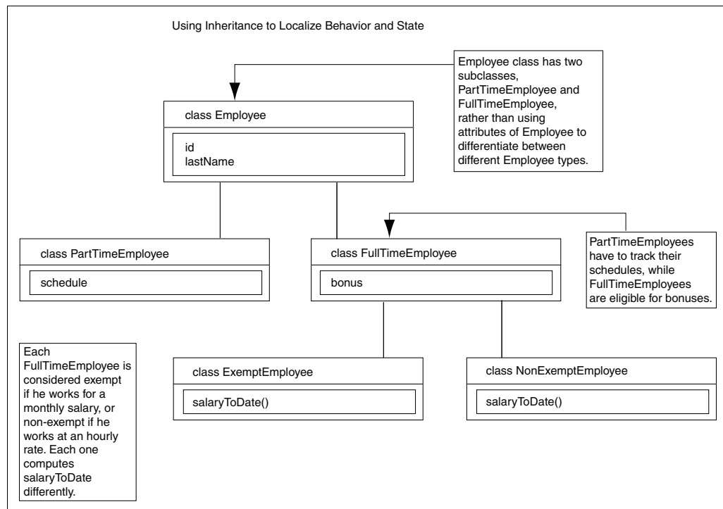
Figure 1-4 Class Hierarchy
