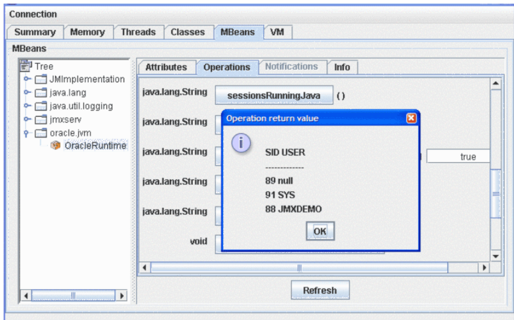
Figure 2-17 Operation sessionsRunningJava
