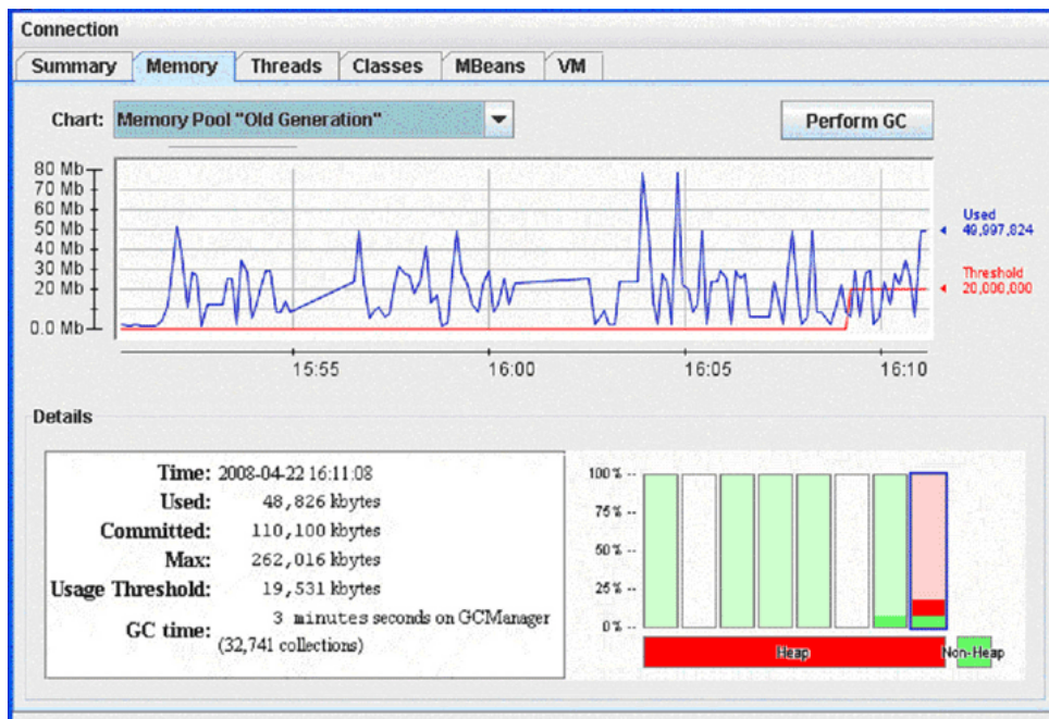
Figure 2-20 Memory Tab of the JConsole Interface When Used Memory Exceeds the Usage Threshold
