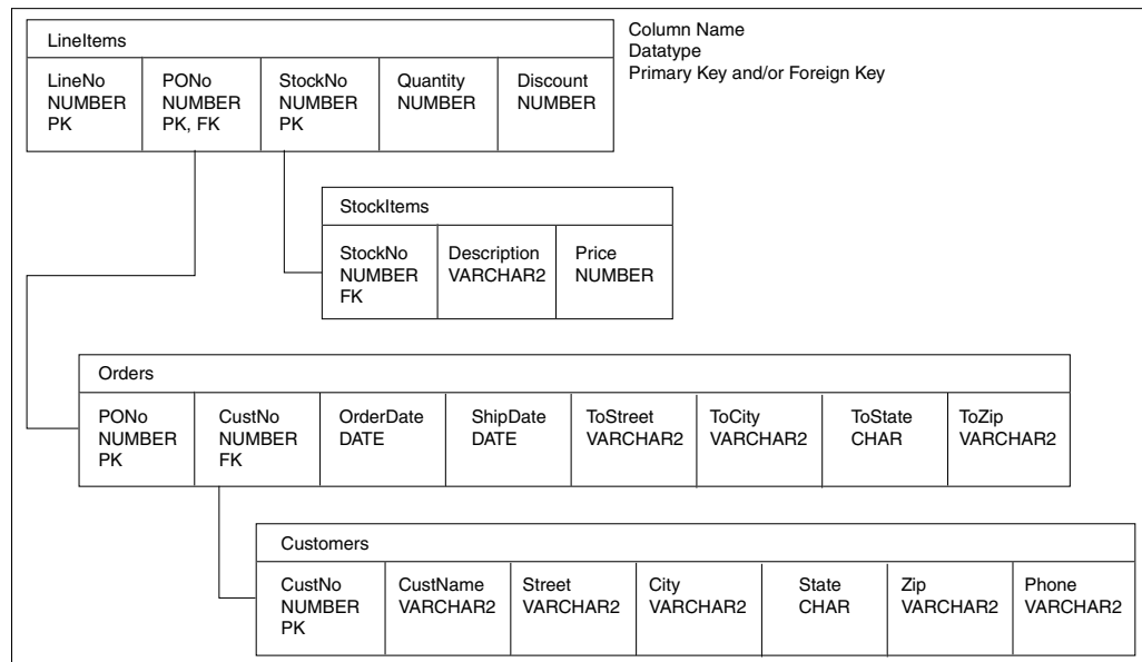
Figure 8-1 Schema Plan for Purchase Order Application
