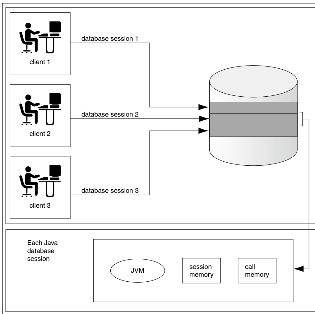
Figure 2-1 Java Environment Within Each Database Session
