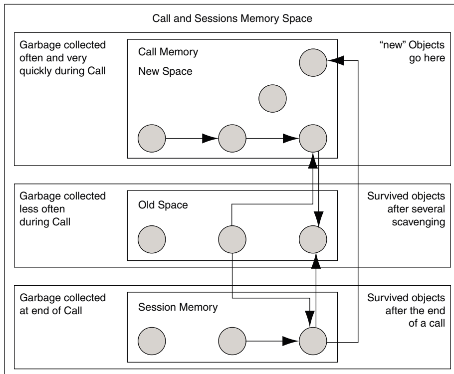
Figure 1-6 Garbage Collection
