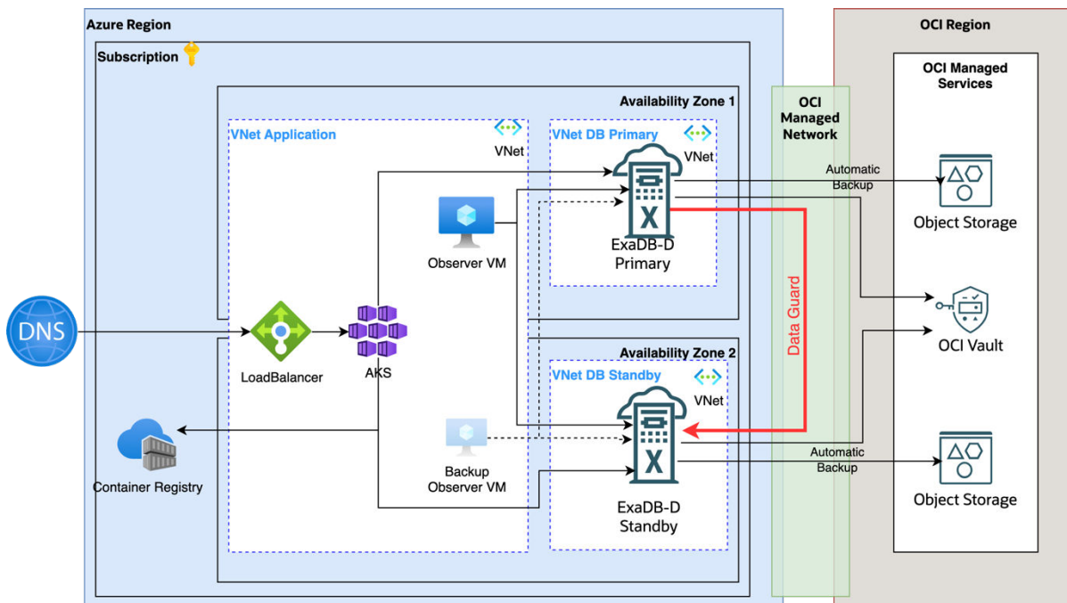
Figure 30-1 DR Capability for a Solution in the Same Region
