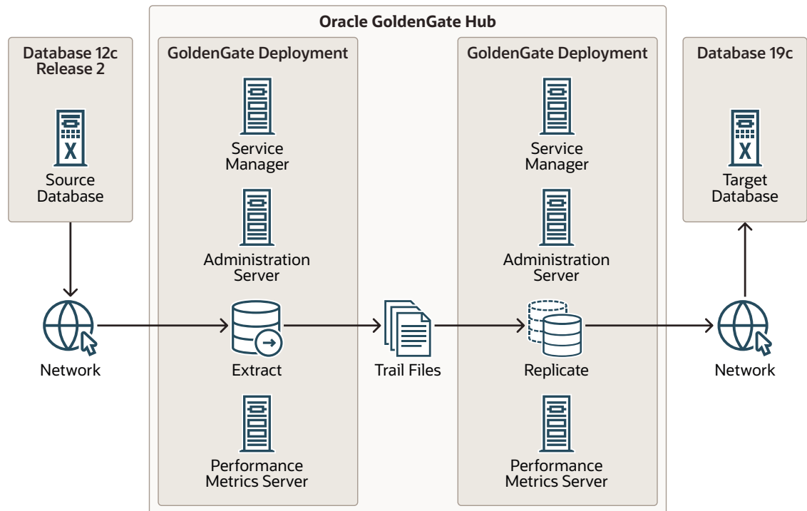
Figure 17-2 MAA Oracle GoldenGate Hub
