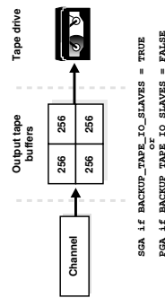
Figure 23-4 Allocation of Tape Buffers
