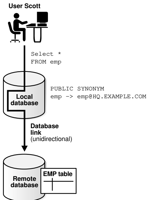
Figure 30-3 Database Link
