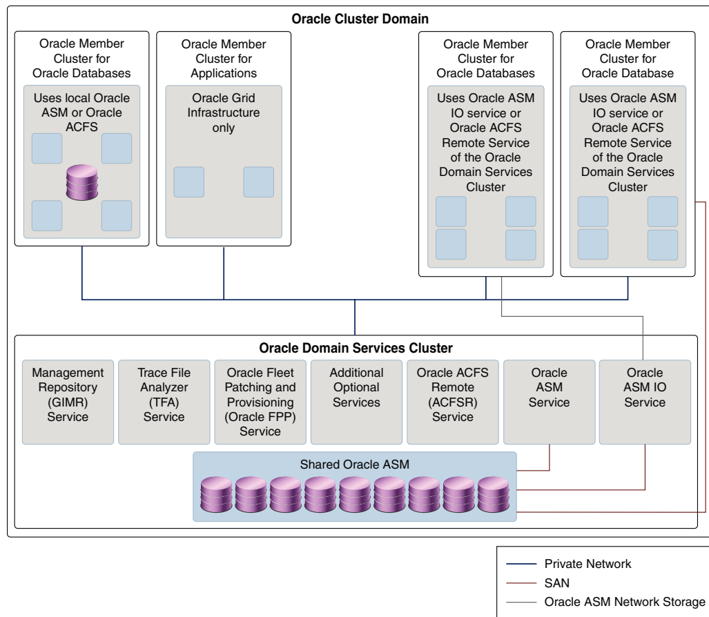
Figure 9-1 Oracle Cluster Domain
