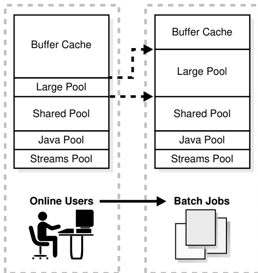
Figure 18-6 Automatic Memory Management
