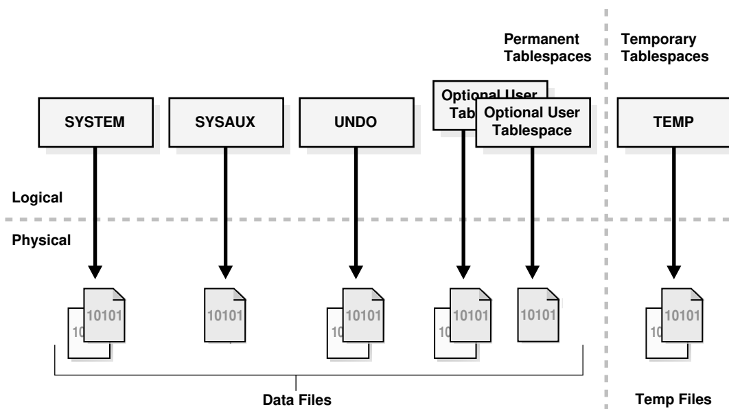
Figure 12-28 Tablespaces
