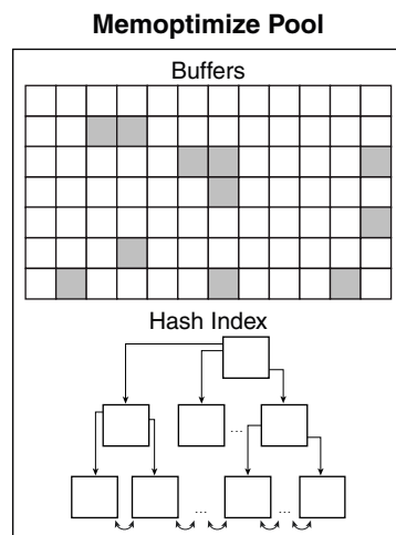
Figure 14-13 Memoptimize Pool
