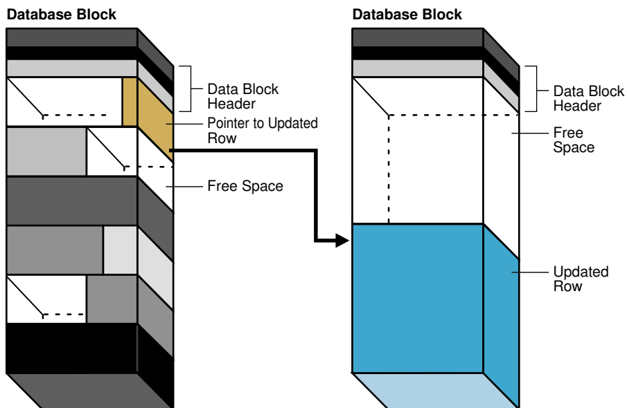
Figure 12-14 Row Migration
