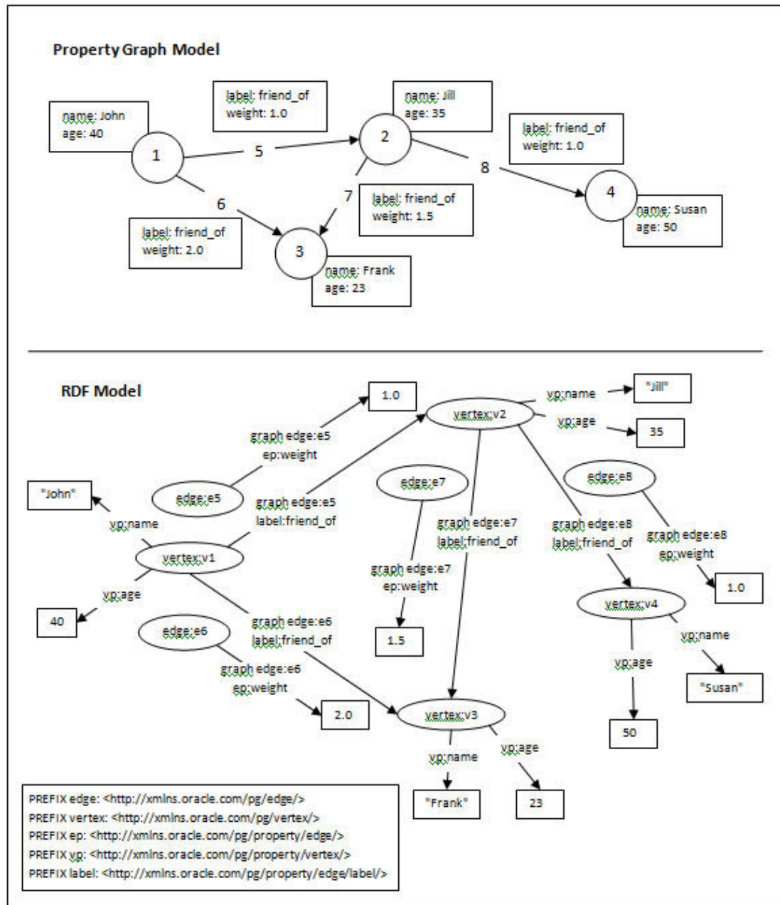
Figure 10-1 Equivalent Property Graph and RDF Representations of the Same Graph
