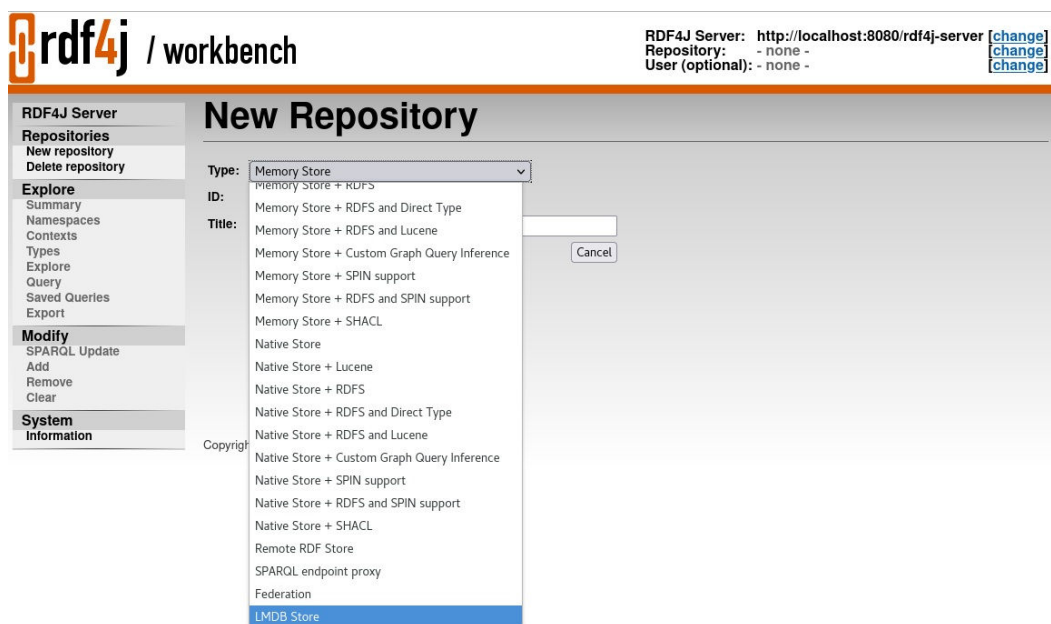
Figure 7-1 Data Source Repository in RDF4J Workbench
