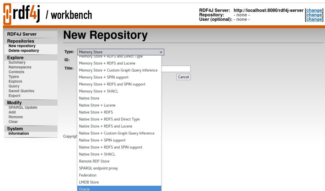
Figure 7-2 RDF4J Workbench Repository
