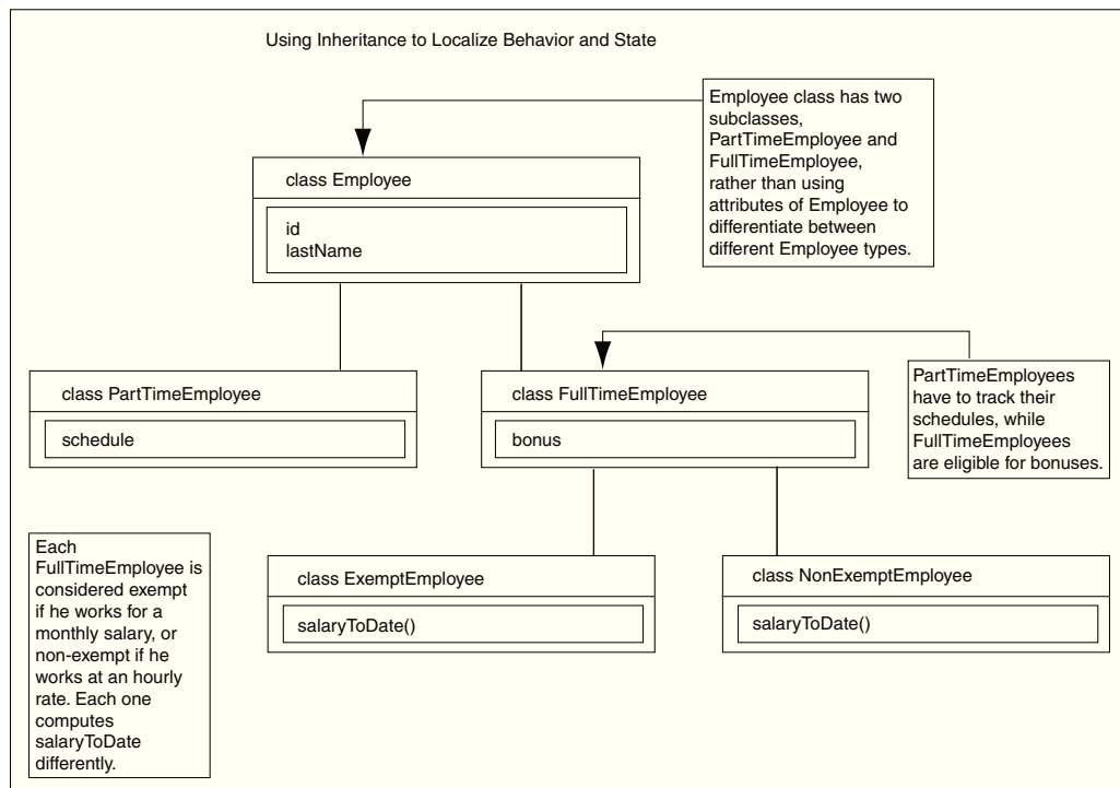
Figure 1-4 Class Hierarchy
