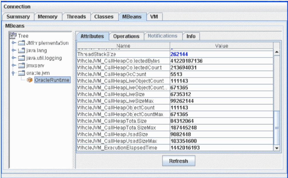
Figure 2-16 OracleRuntime MBean
