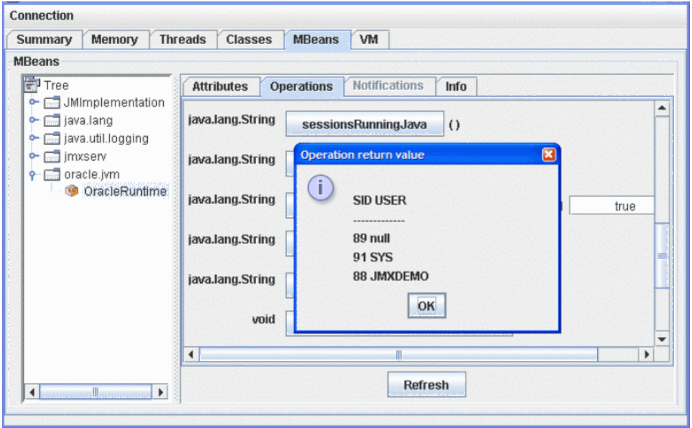
Figure 2-17 Operation sessionsRunningJava
