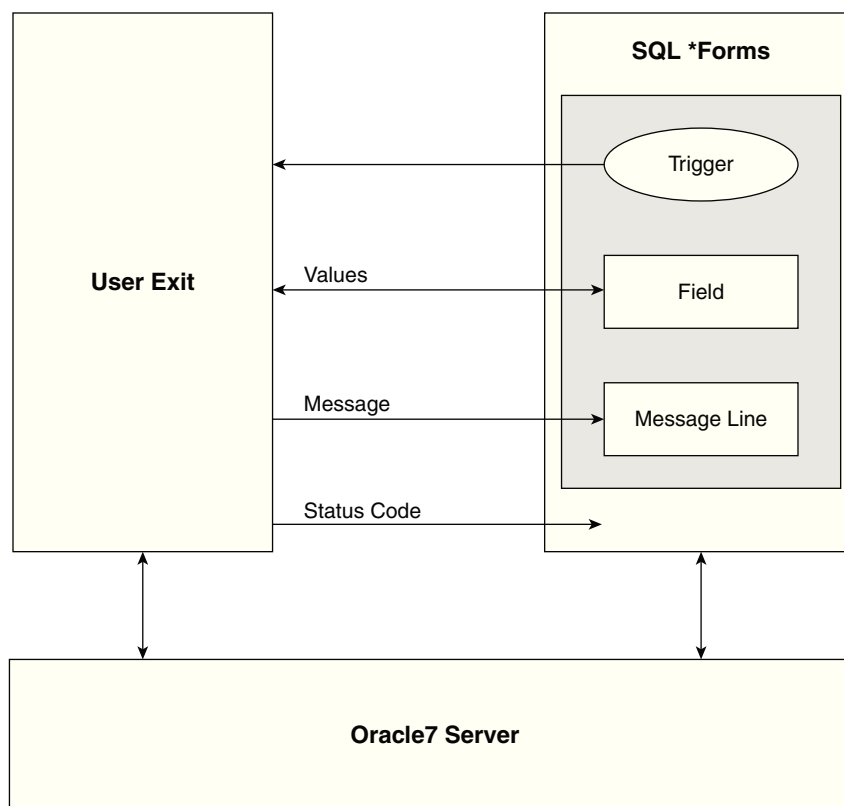
Figure 11-1 SQL*Forms
