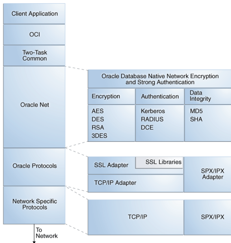
Figure 15-3 Oracle Native Network Encryption and Strong Authentication Architecture
