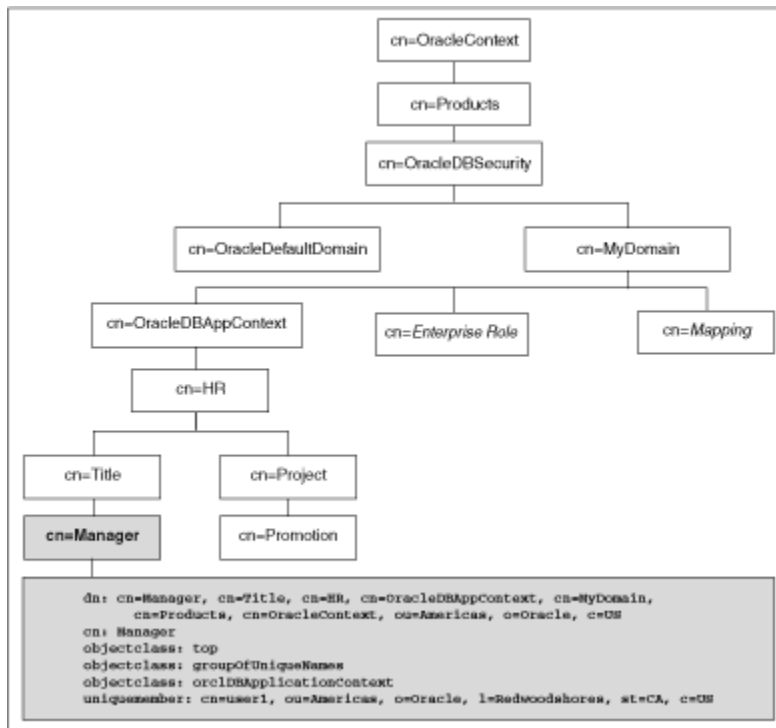
Figure 9-1 Location of Application Context in LDAP Directory Information Tree
