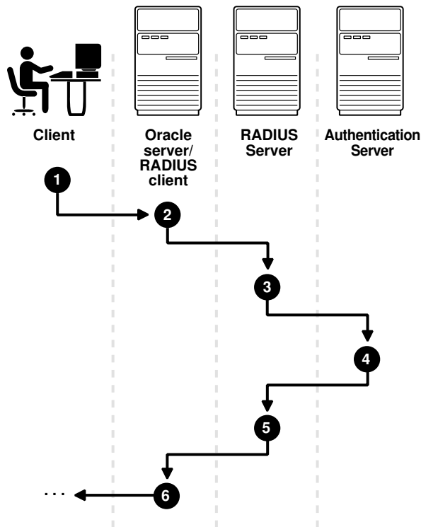
Figure 19-2 Synchronous Authentication Sequence
