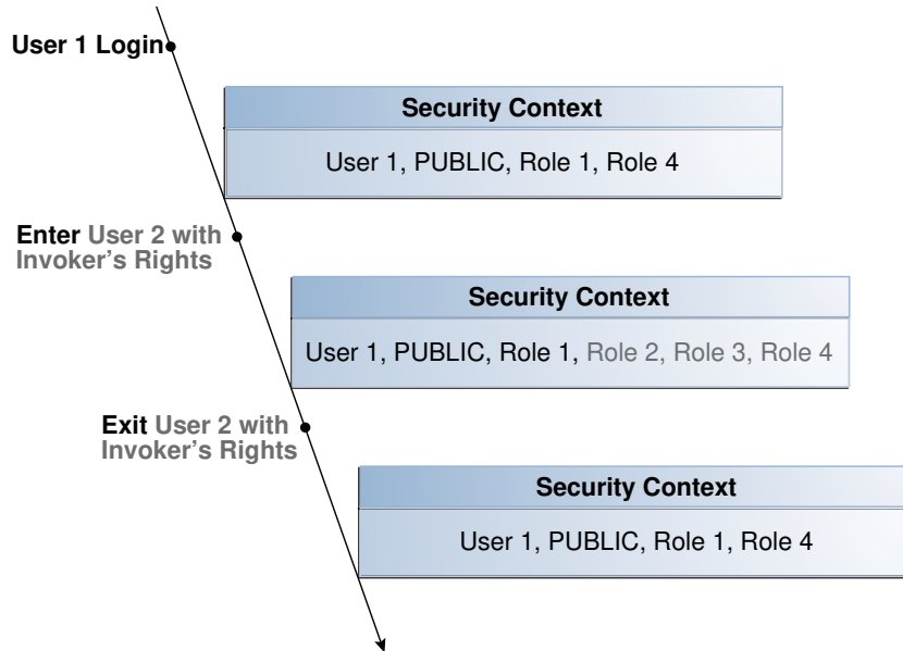
Figure 5-2 Security Context in Which Invoker's Right Program Unit IR Is Executed
