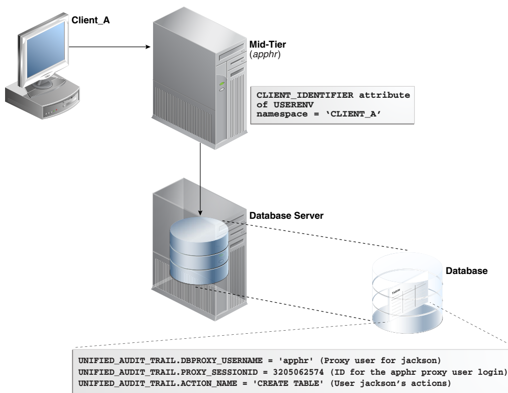
Figure 22-1 Auditing Proxy Users
