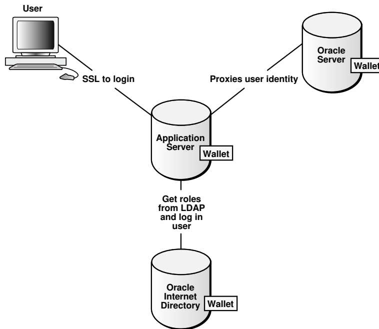
Figure 3-2 Multitier Authentication
