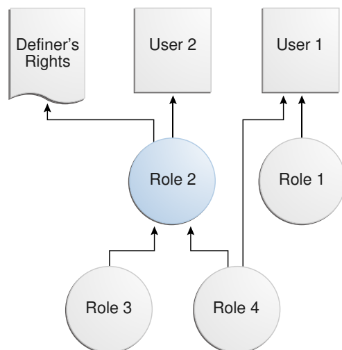
Figure 5-3 Roles Granted to Application Users and Definer's Rights Program Unit
