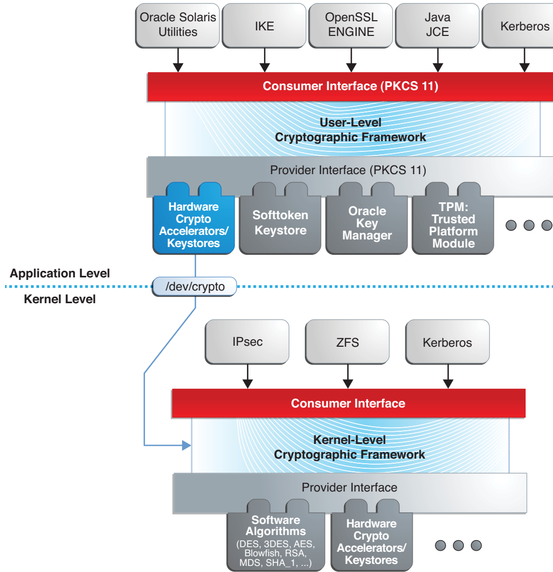
FIGURE 8-1 Overview of the Oracle Solaris Cryptographic Framework
