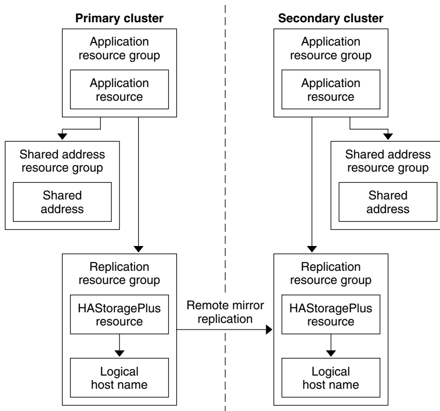
FIGURE A-5 Configuration of Resource Groups in a Scalable Application
