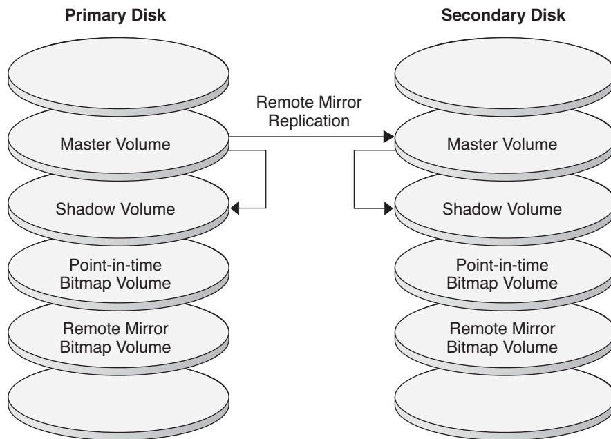
FIGURE A-3 Replication in the Example Configuration
