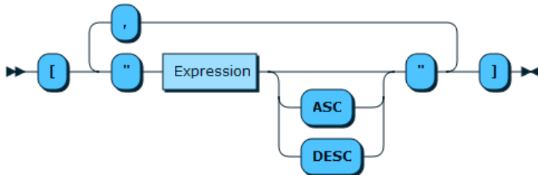
Figure 11.28 SortExprStrList
