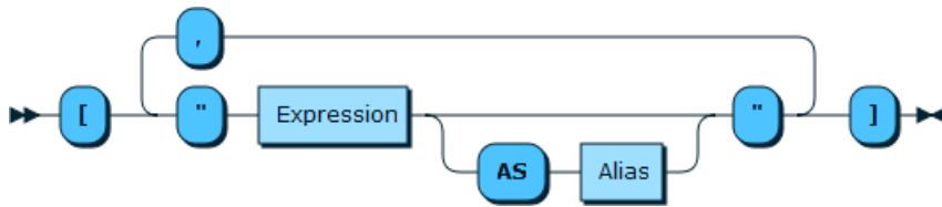
Figure 11.27 ProjectedSearchExprStrList
